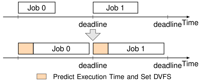
Figure 4.4: Operation of predictive DVFS.
