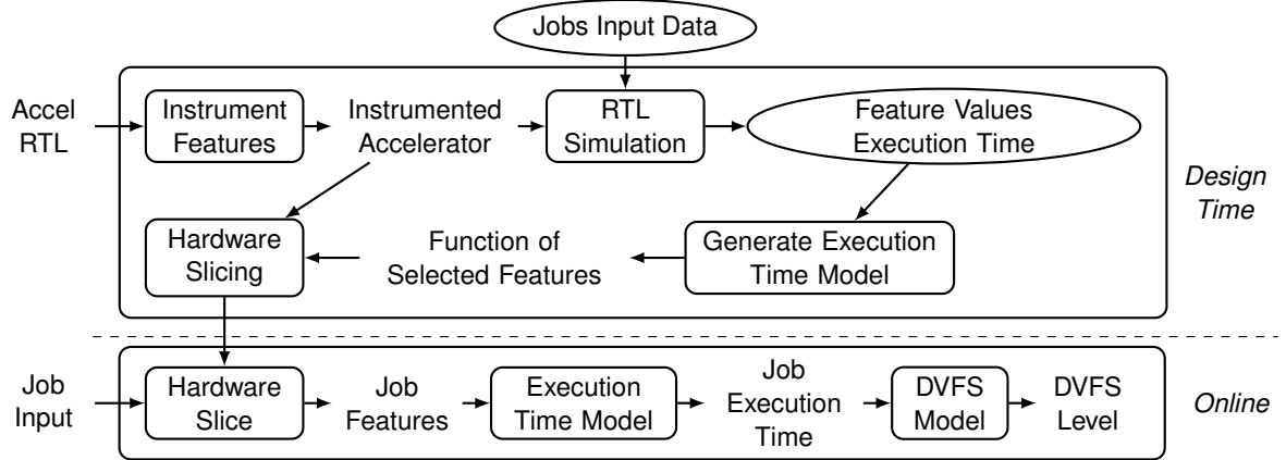
Figure 4.6: Execution time prediction flow.
