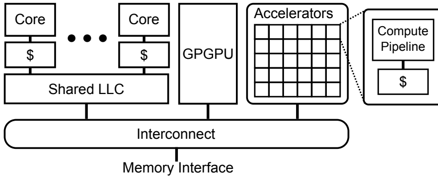
Figure 2.1: System architecture.
