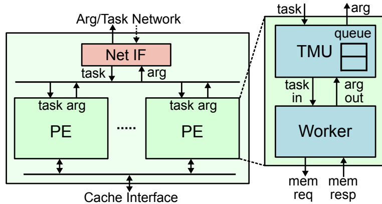
Figure 3.6: LiteArch tile.
