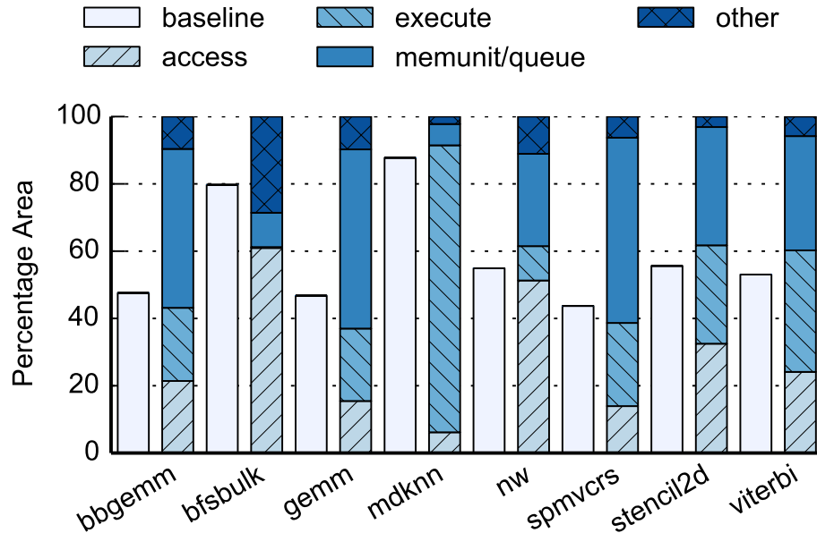
Figure 2.12: Area breakdown of DAE accelerators. The baseline area is shown for comparison.
