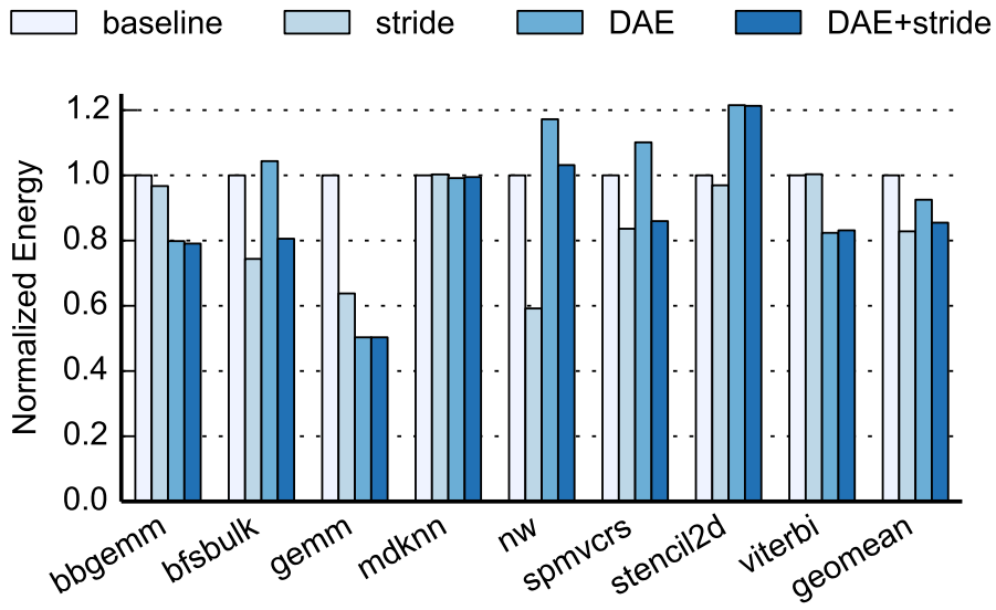
Figure 2.14: Energy comparison.
