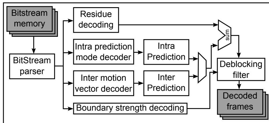
Figure 4.10: Architecture of H.264 decoder.
