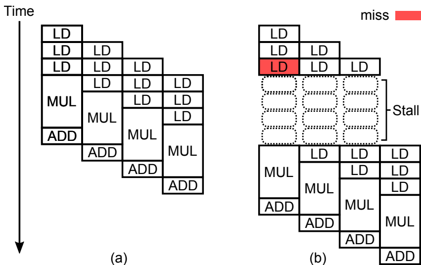
Figure 2.4: Example schedule of an HLS SpMV accelerator with (a) ideal memory (b) cache that has a miss when accessing vec .
