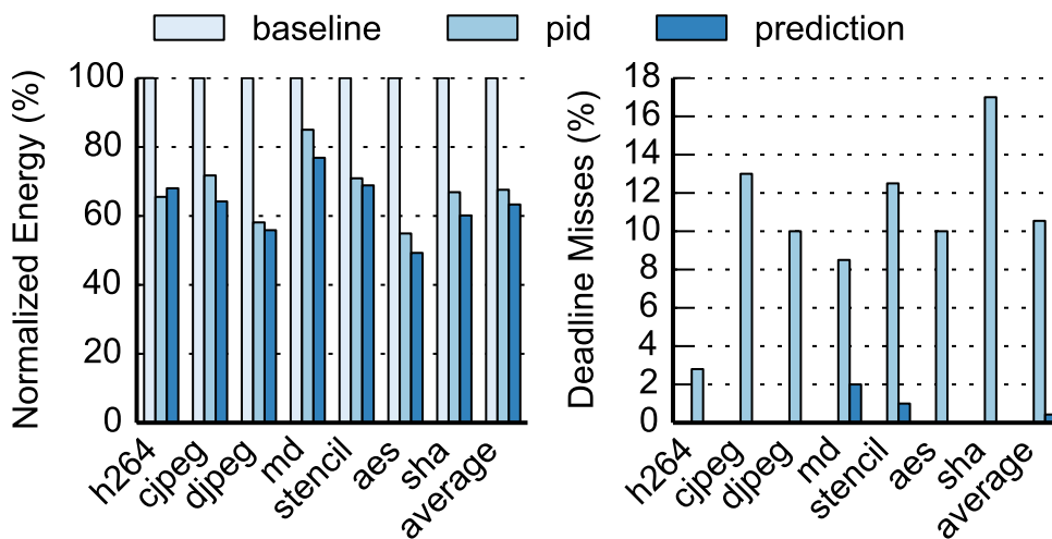
Figure 4.12: Normalized energy and deadline misses of different DVFS schemes.
